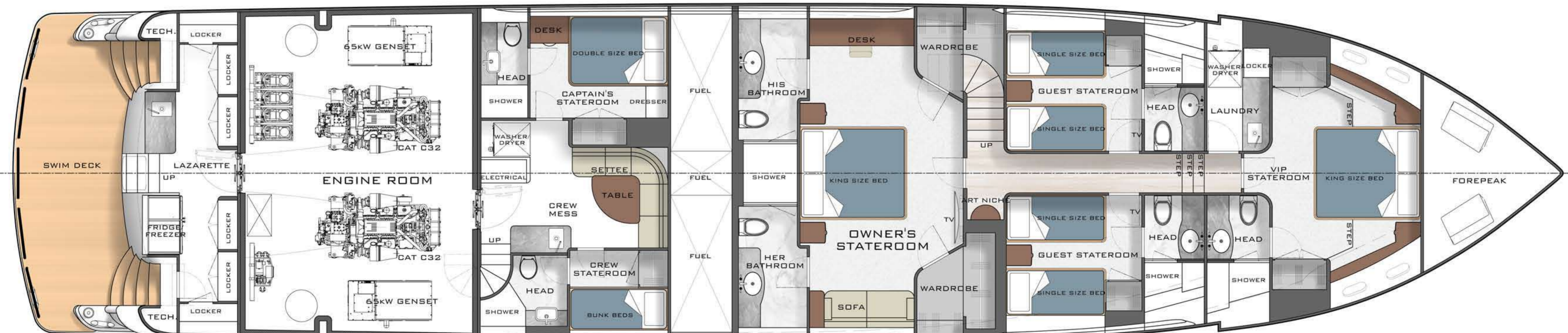
HULL DECK
